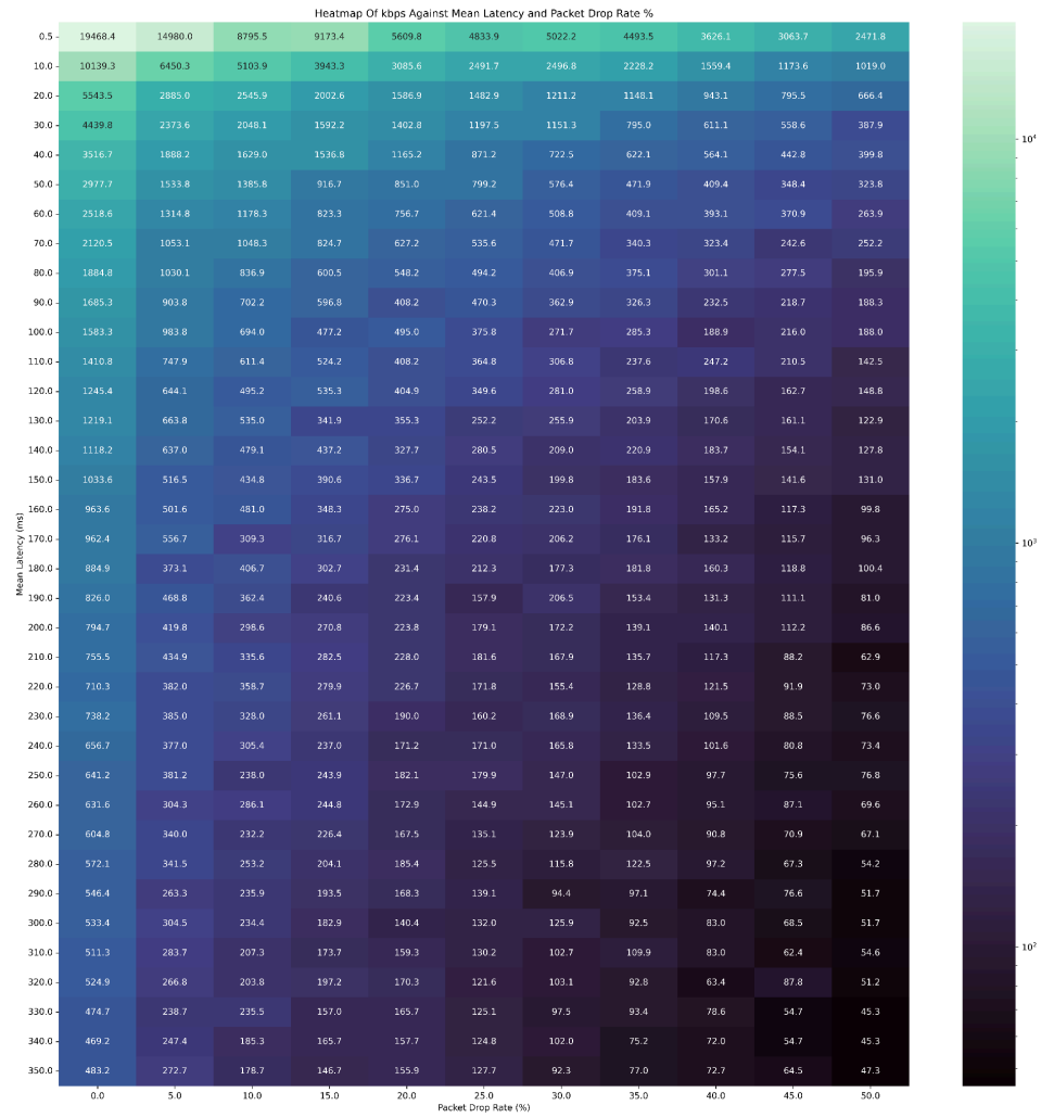
Heatmap showing average kbps against mean latency and packet drop rate
